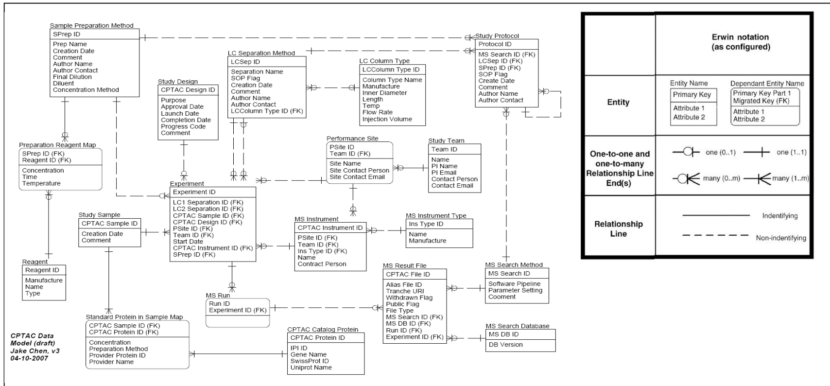
Relational data model schema of CPTAC data management. The figure legend is shown in the upper right.
